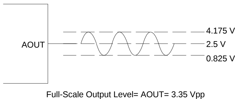
Figure 19. Full-Scale Output
