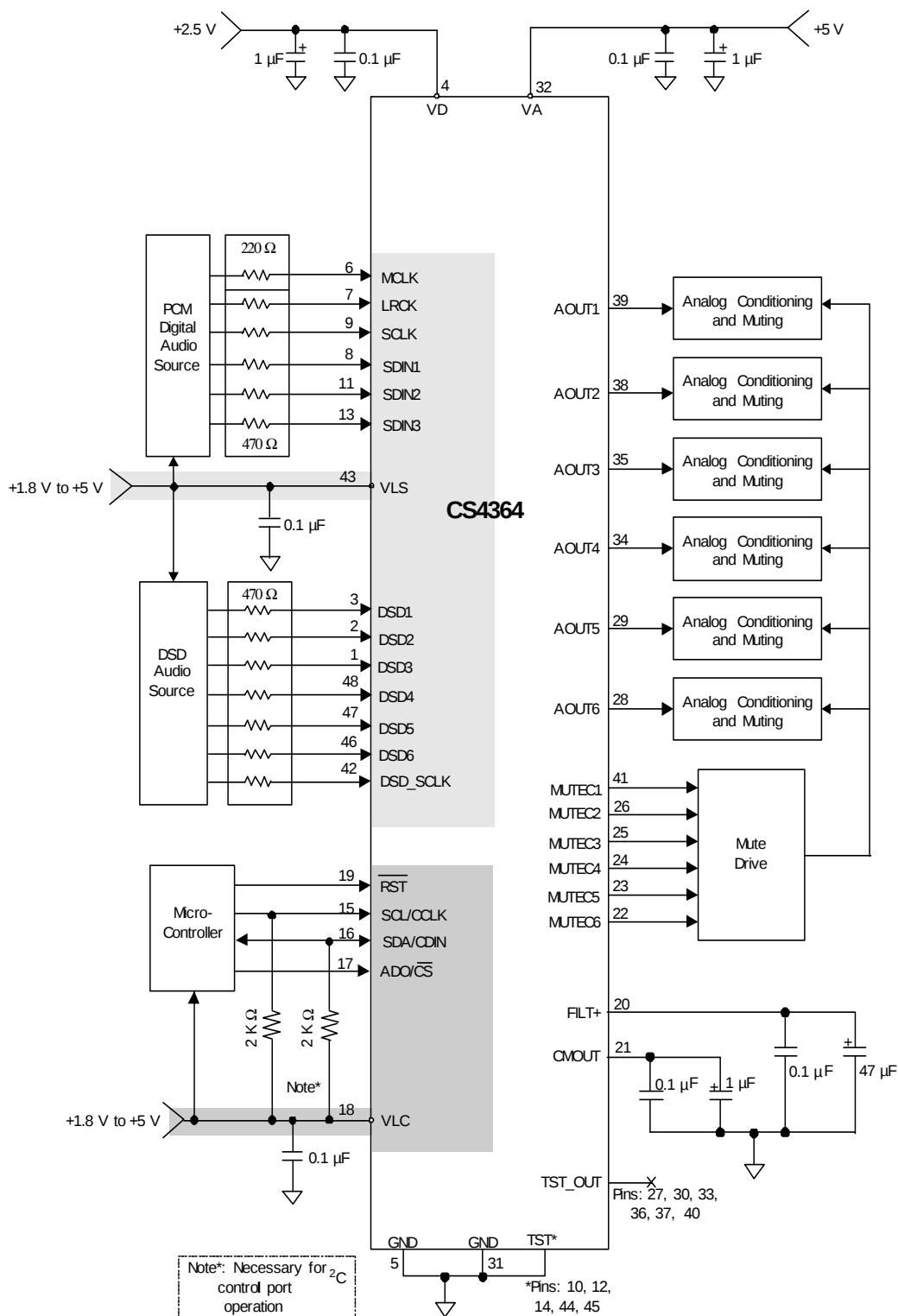
Figure 6. Typical Connection Diagram, Software Mode
